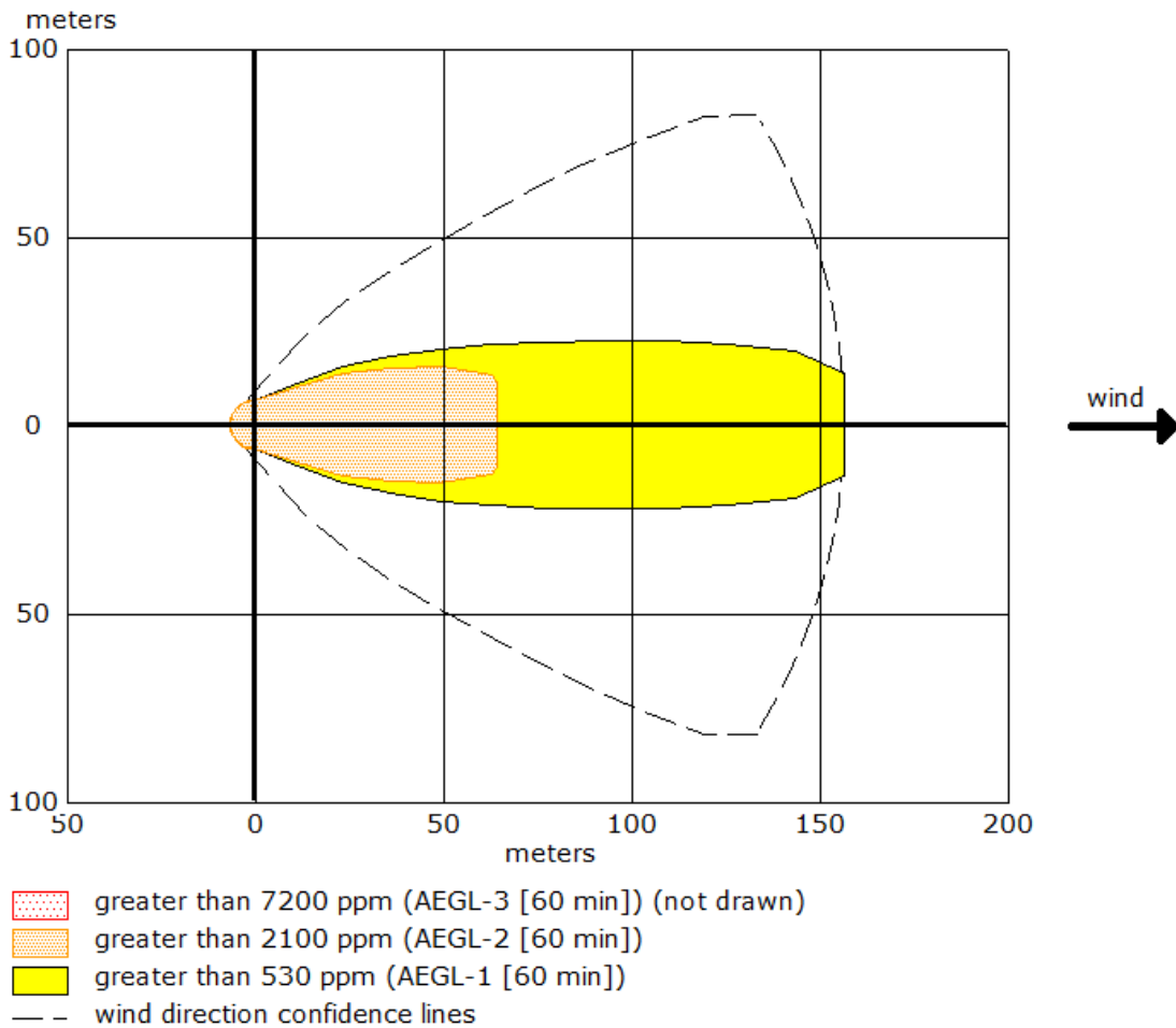
Figure 8-1: Scenario: Leaking tank, chemical is not burning and forms an evaporating puddle
