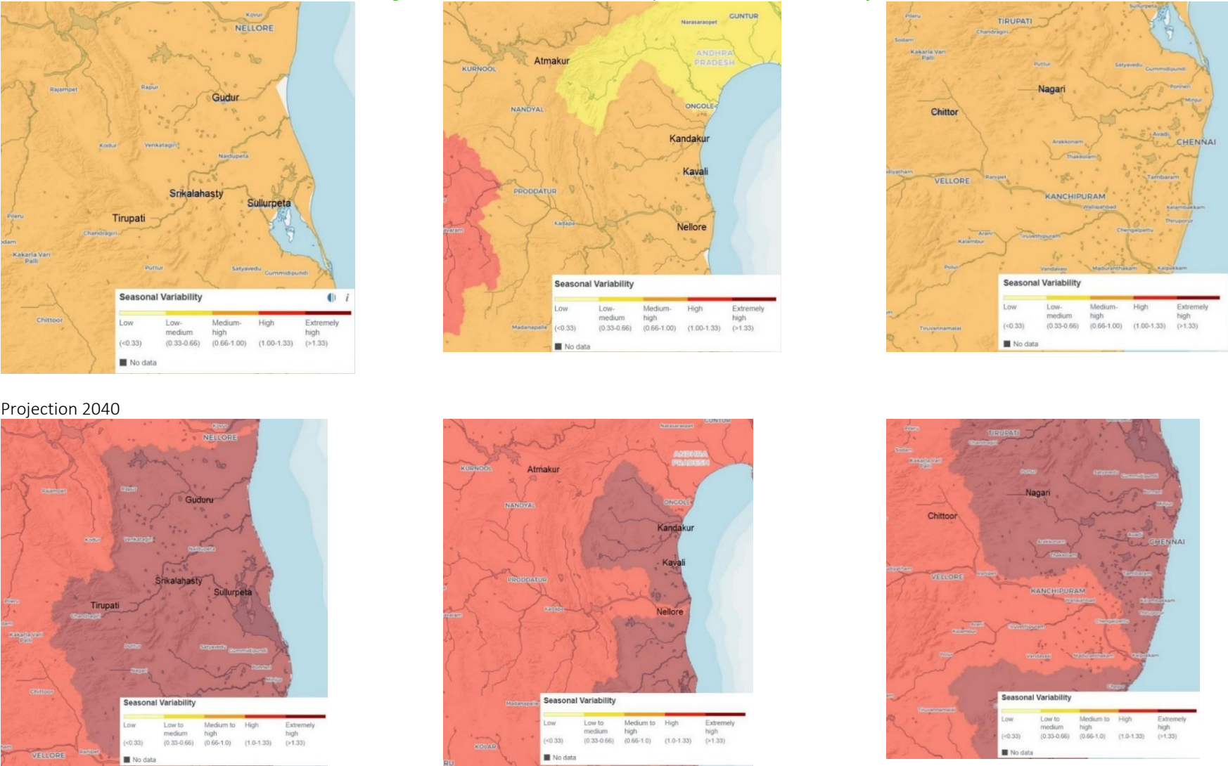
Figure 4-16: Seasonal Variability – Current Scenario and Projection 2040
