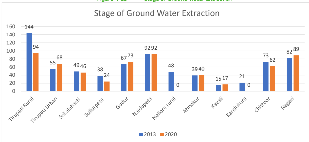
Figure 4-13 Stage of Ground water Extraction
