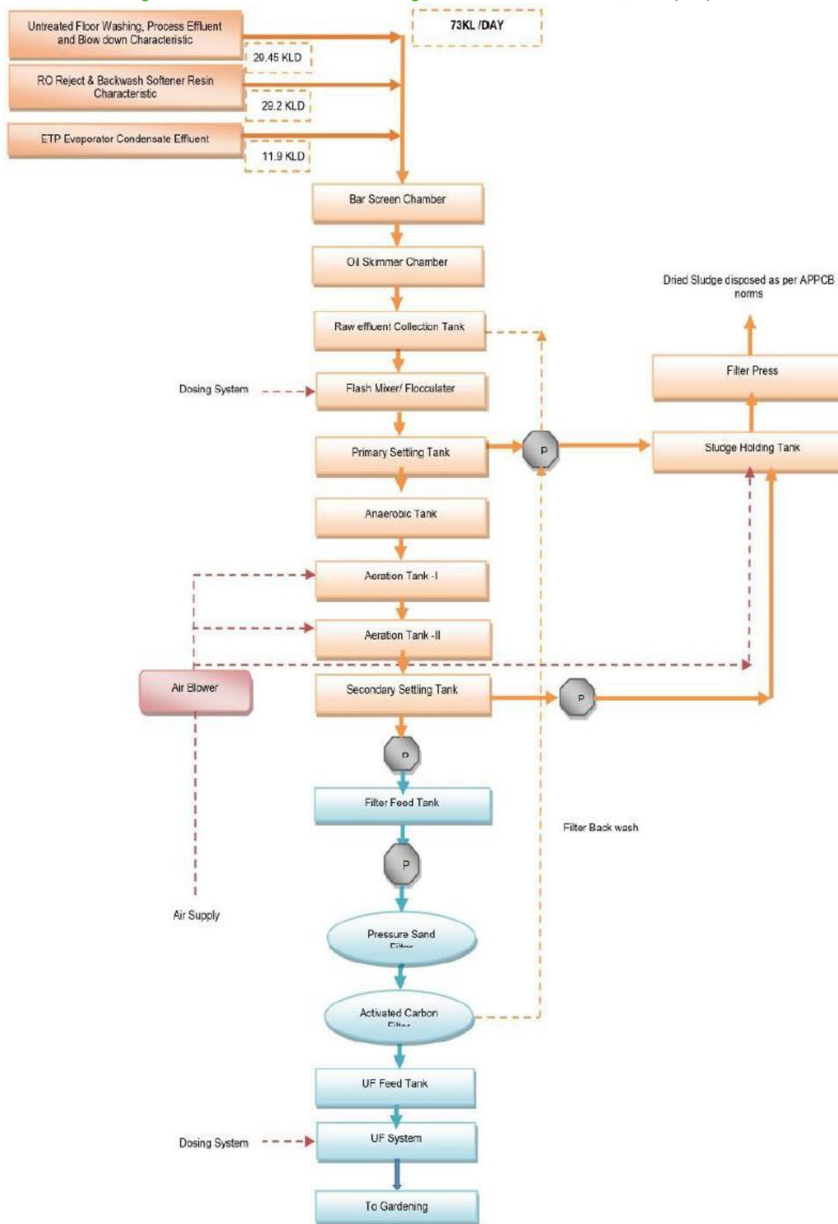
Figure 2-5: Schematic Flow Diagram for Effluent Treatment Plant (ETP)
